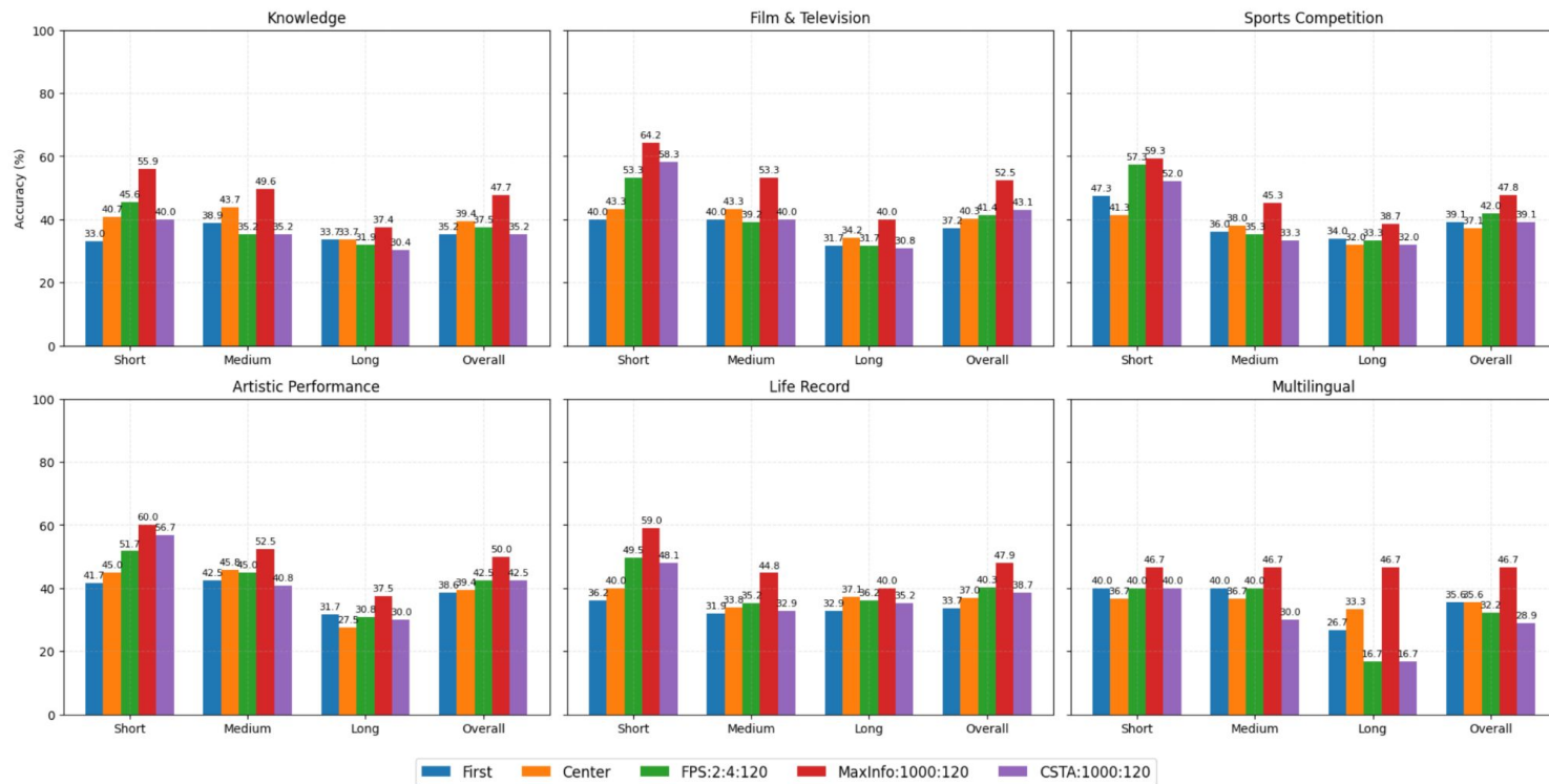
SmolVLM performance on VideoMME for Video Categories and Sampling Techniques
